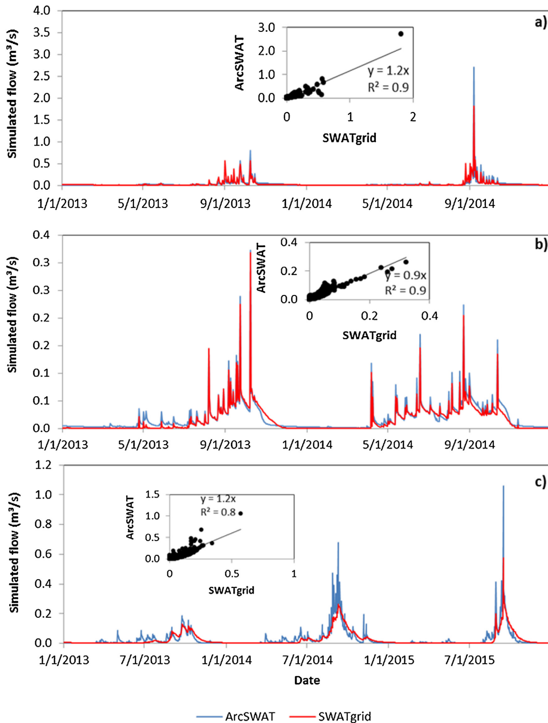
Fig. 6. Comparison of flow (m 3 /s) simulated by ArcSWAT and SWATgrid, and corresponding scattergrams at the outlets of (a) Kounga (from 2013 to 2014), (b) Kpandouga (from 2013 to 2014), and (c) Tossahou (from 2013 to 2015).
