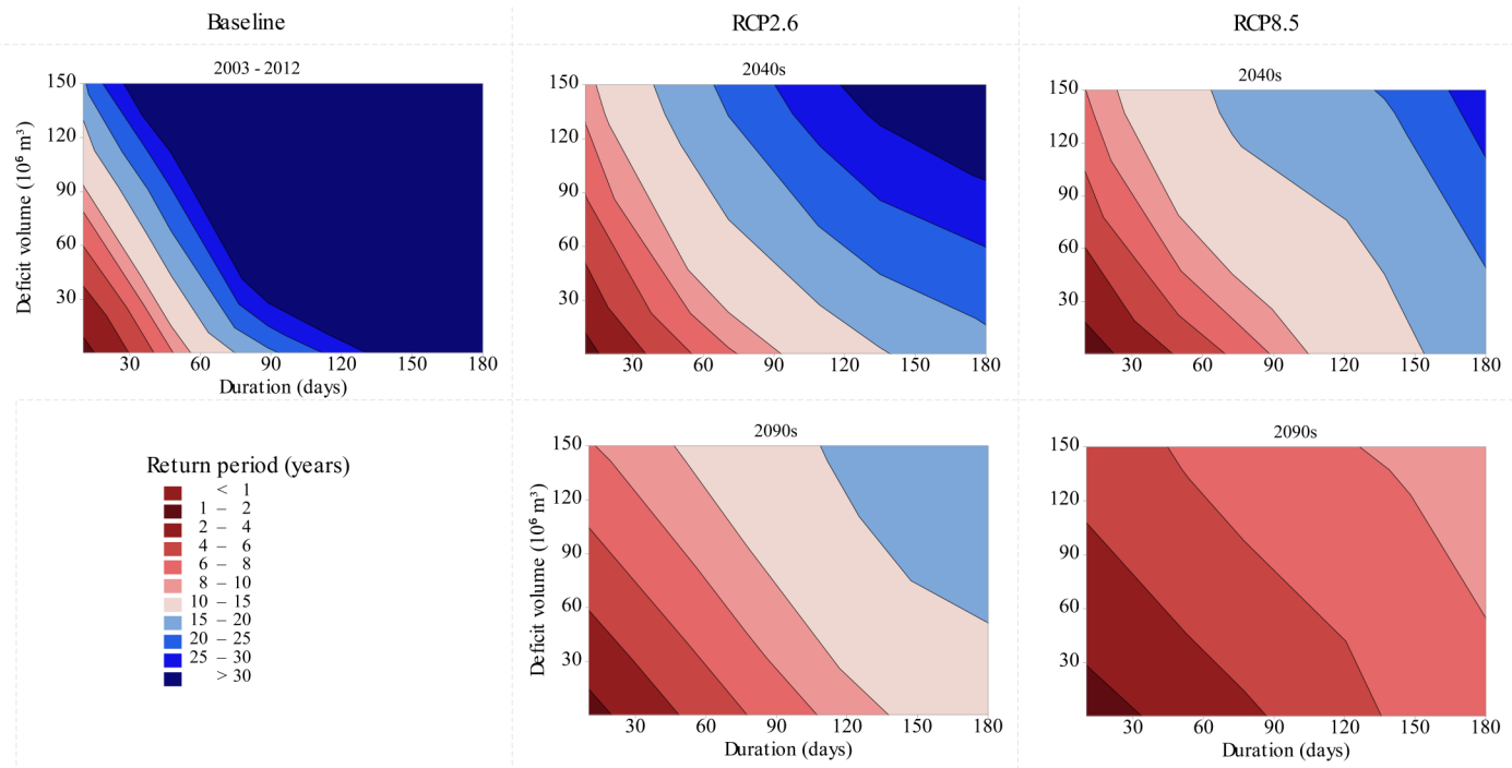
Fig 6. Contour plots showing severity-duration-frequency relationships of streamflow droughts in the Upper Ouémé watershed under baseline climatic conditions (2003–2012) and two RCP scenarios. Contour plots were derived using daily streamflow simulated at the watershed outlet.
